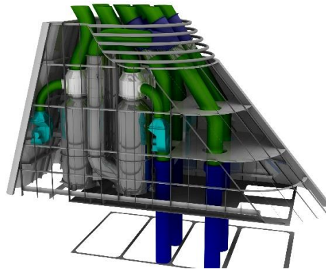
Hybrid scrubber system – funnel structure
